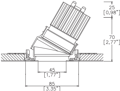
Mix85 Edge with Trimless Kit TL2 (1) (rear fitting, partial skim) Cut-out Ø90mm Required depth height + 25mm.
