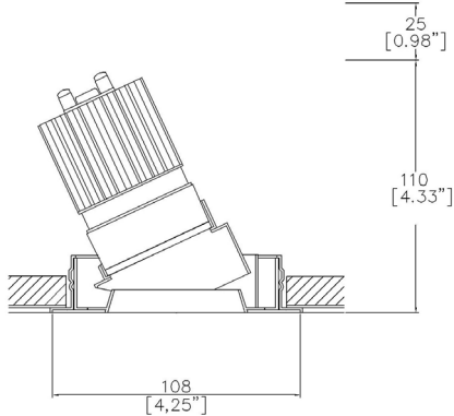
A31603-LED + 3000-PCZ 359° rotation. Up to 35° tilt. Cut-out 98mm (3.85”) Ø
