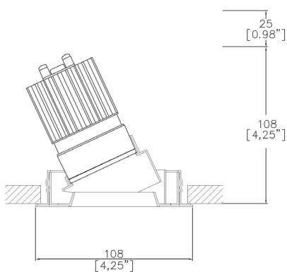
A31603-LED + 3000-PBZ 359° rotation. Up to 35° tilt. Cut-out 103mm (4.00”) Ø
