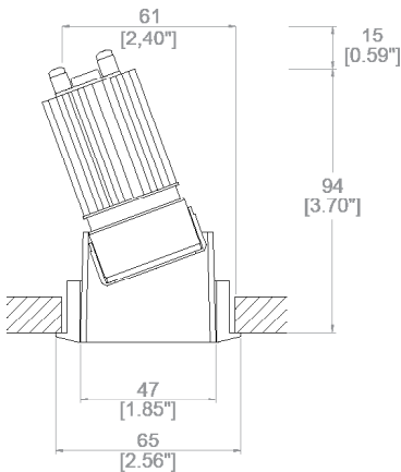
050-LED-TR Cut-out Ø 61mm Required depth height + 15mm^
