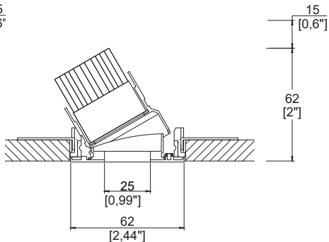
Mix60 Edge with Trimless Kit TL3 (1) (rear fitting, solid ceiling) Cut-out Ø61mm. Required depth height + 15mm.
