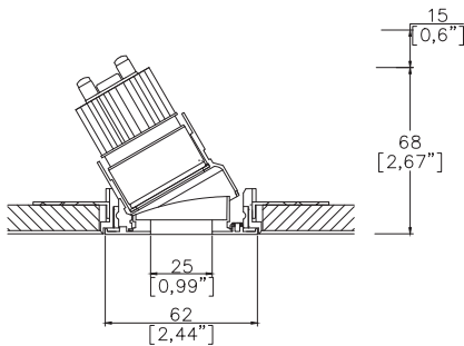
Mix60 Edge with Trimless Kit TL2 (1) (rear fitting, partial skim) Cut-out Ø66mm. Required depth height + 15mm.
