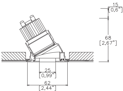
Mix60 Edge with Trimless Kit TL1 (1) (front fitting, full skim) Cut-out Ø68mm. Required depth height + 15mm.
