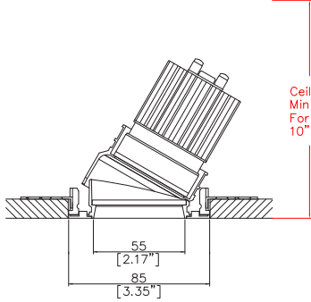
Mix85 Duo with Trimless Kit TL3 (1) (rear fitting, solid ceiling) Cut-out Ø3.39" (86mm)
