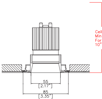
Mix85 Duo with Trimless Kit TL1 (1) (front fitting, full skim) Cut-out Ø3.54” (90mm)
