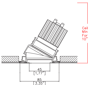
Mix85 Edge with Trimless Kit TL1 (1) (front fitting, full skim) Cut-out Ø3.54" (90mm)
