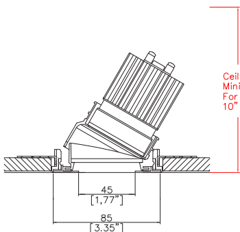
Mix85 Edge with Trimless Kit TL2 (1) (rear fitting, partial skim) Cut-out Ø3.54" (90mm)
