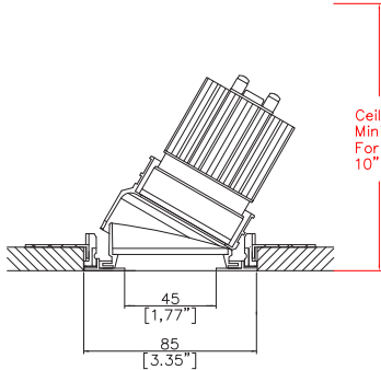
Mix85 Edge with Trimless Kit TL3 (1) (rear fitting, solid ceiling) Cut-out Ø3.39" (86mm)
