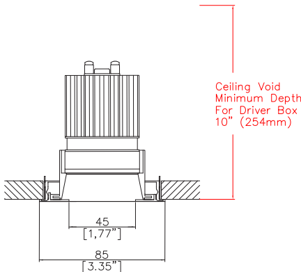
Mix85 Edge with Trim Kit TR1 (1) Cut-out Ø3.15” (80mm).
