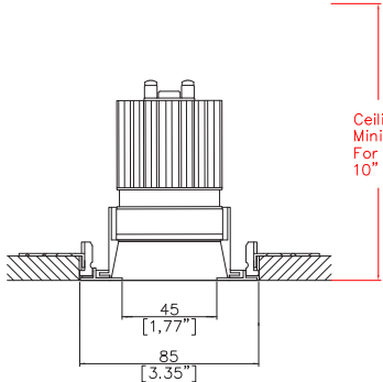
Mix85 Edge with Trimless Kit TL3 (1) (rear fitting, solid ceiling) Cut-out Ø3.39” (86mm)
