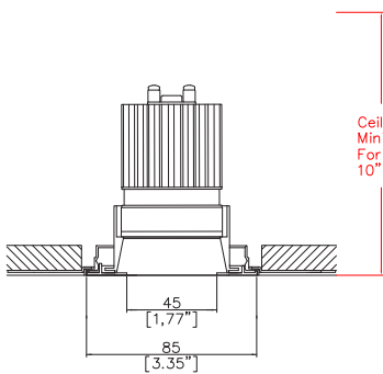
Mix85 Edge with Trimless Kit TL1 (1) (front fitting, full skim) Cut-out Ø3.54” (90mm)
