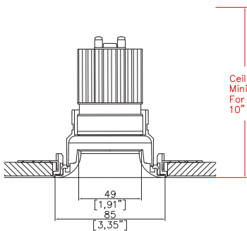
Mix85 Flare with Trimless Kit TL2 (1) (rear fitting, partial skim) Cut-out Ø3.54” (90mm)
