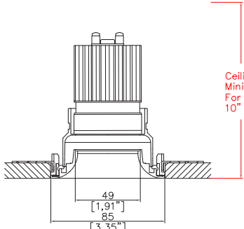
Mix85 Flare with Trimless Kit TL3 (1) (rear fitting, solid ceiling) Cut-out Ø3.39” (86mm)
