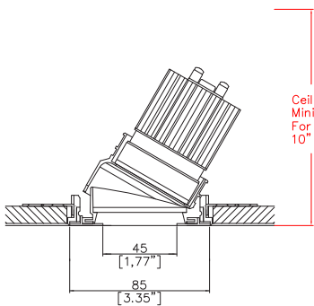
Mix85 Pinhole with Trimless Kit TL2 (1) (rear fitting, partial skim) Cut-out Ø3.54" (90mm)
