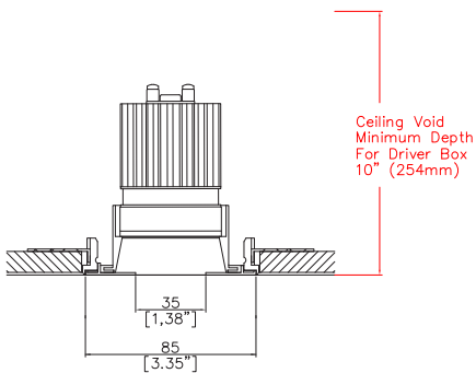
Mix85 Pinhole with Trimless Kit TL2 (1) (rear fitting, partial skim) Cut-out Ø3.54” (90mm)
