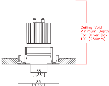
Mix85 Pinhole with Trimless Kit TL3 (1) (rear fitting, solid ceiling) Cut-out Ø3.39” (86mm)
