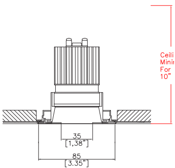
Mix85 Pinhole with Trimless Kit TL1 (1) (front fitting, full skim) Cut-out Ø3.54” (90mm)
