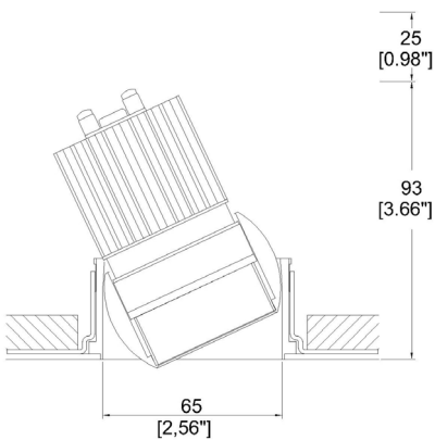
Oculus with Trimless. Kit TL1 (1) (front fitting, full skim) Cut-out Ø82mm (Ø3,22").
