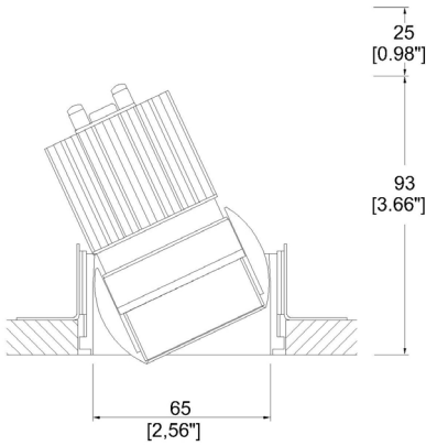
Oculus with Trimless. Kit TL2 (1) (rear fitting, partial skim) Cut-out Ø81mm (Ø3,19").
