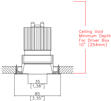
Mix85 Pinhole with Trim Kit TR1 (1) Cut-out Ø3.15” (80mm).
