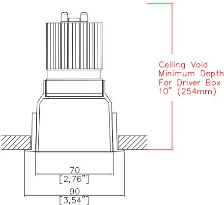
ASF70100-TR1 Cut-out Ø 3.22” (82mm)
