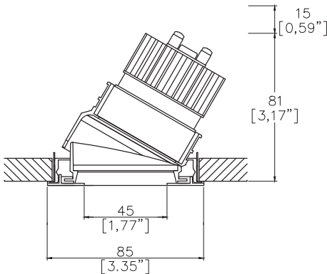
Mix85 Edge with Trim Kit TR1 (1) Cut-out Ø80mm. Required depth height+15mm.
