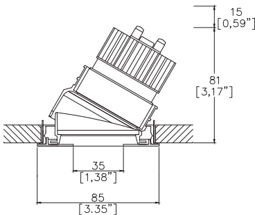
Mix85 Pinhole with Trim Kit TR1 (1) Cut-out Ø80mm. Required depth height+15mm.
