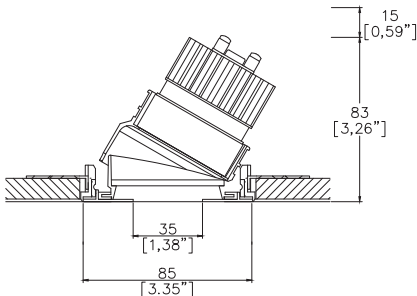
Mix85 Pinhole with Trimless Kit TL2 (1) (rear fitting, partial skim) Cut-out Ø90mm Required depth height + 15mm.
