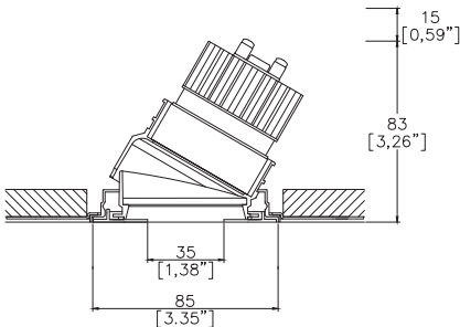
Mix85 Pinhole with Trimless Kit TL1 (1) (front fitting, full skim) Cut-out Ø90mm Required depth height + 15mm.
