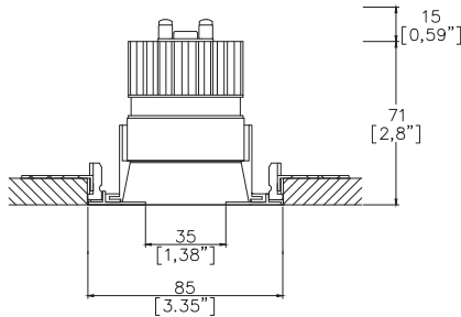
Mix85 Pinhole with Trimless Kit TL3 (1) (rear fitting, solid ceiling) Cut-out Ø86mm Required depth height +15mm.
