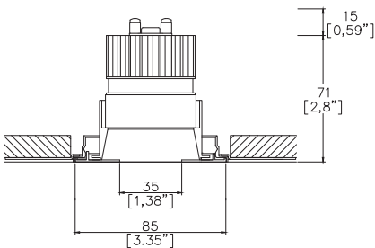
Mix85 Pinhole with Trimless Kit TL1 (1) (front fitting, full skim) Cut-out Ø90mm Required depth height + 15mm.
