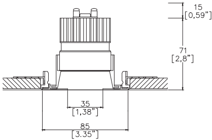
Mix85 Pinhole with Trimless Kit TL2 (1) (rear fitting, partial skim) Cut-out Ø90mm Required depth height + 15mm.
