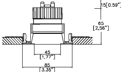
Mix85 Edge with Trimless Kit TL3 (1) (rear fitting, solid ceiling) Cut-out Ø86mm Required depth height + 25mm.
