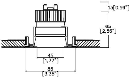
Mix85 Edge with Trimless Kit TL2 (1) (rear fitting, partial skim) Cut-out Ø90mm Required depth height + 25mm.
