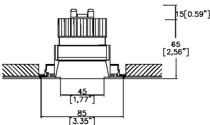
Mix85 Edge with Trimless Kit TL1 (1) (front fitting, full skim) Cut-out Ø90mm Required depth height + 25mm.
