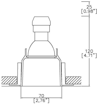
070-GU-TL Cut-out 79mm Ø
