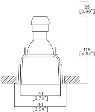
070-GU-TR Cut-out 79mm Ø
