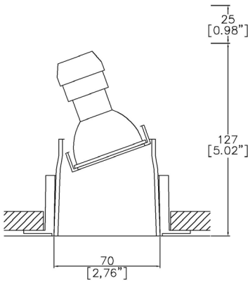
073-GU-TL Cut-out 79mm Ø
