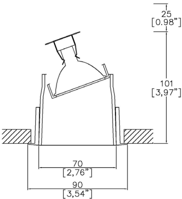
073-MR-TR Cut-out 79mm Ø
