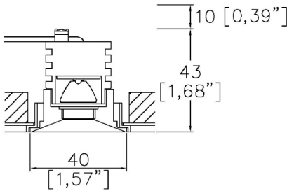
AM40-CL-TL Cut-out 37mm (1.46”) Ø
