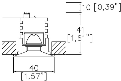
AM40-CL-TR Cut-out 36mm (1.42”) Ø
