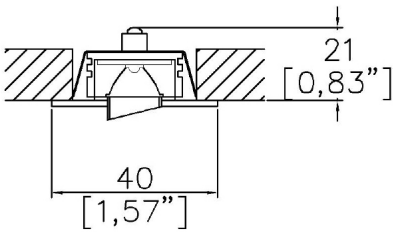
AM40-MD Cut out Ø27mm
