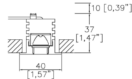
AM40-PE-TR Cut-out 36mm (1.42”) Ø
