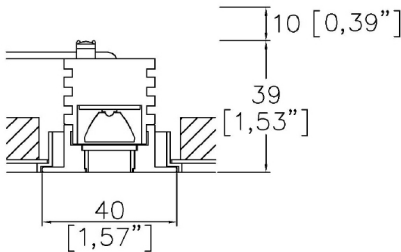
AM40-PE-TL Cut-out 37mm (1.46”) Ø
