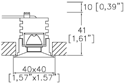
M40-PY-TR Cut-out 37 x 37mm (1.46” x 1.46”)
