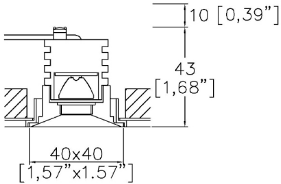
M40-PY-TL Cut-out 38 x 38mm (1.50” x 1.50”)
