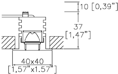
M40-SE-TR Cut-out 37 x 37mm (1.46" x 1.46")
