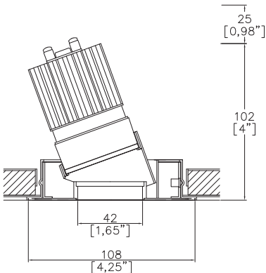
A31413-A-LED + 3000-PCZ 360° rotation. Up to 30° tilt. Cut-out 98mm (3.85”) Ø
