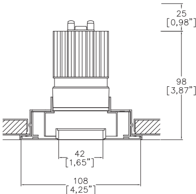
A31413-F-LED + 3000-PCZ Cut-out 98mm (3.85”) Ø
