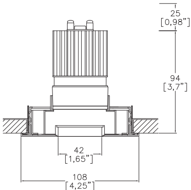
A31413-F-LED + 3000-PBZ Cut-out 103mm (4.00”) Ø
