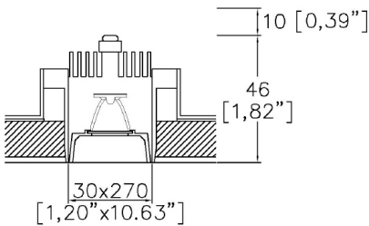
A2610-CB-TL Cut out 272 x 35mm (10.71" x 1.38")
