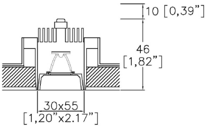
A2602-CB-TL Cut out 59 x 35mm (2.32" x 1.38")
