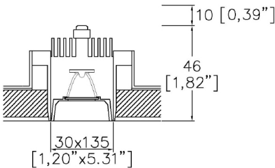
A2605-CB-TL Cut out 139 x 35mm (5.47" x 1.38")
