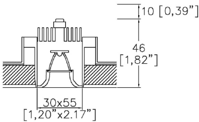
A2602-FL-TL Cut out 59 x 35mm (2.32" x 1.38")
